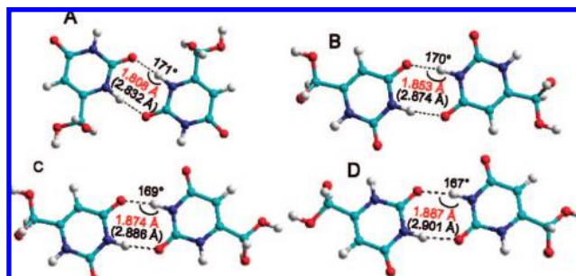
Figure 2. N—H...O hydrogen bonding within a plane for the dimers A, B, C and D, respectively. Color coding: C, cyan; O, red; N, blue; H, white. NH...O angle, H...O (in red) and N...O distances (in brackets) are indicated.
